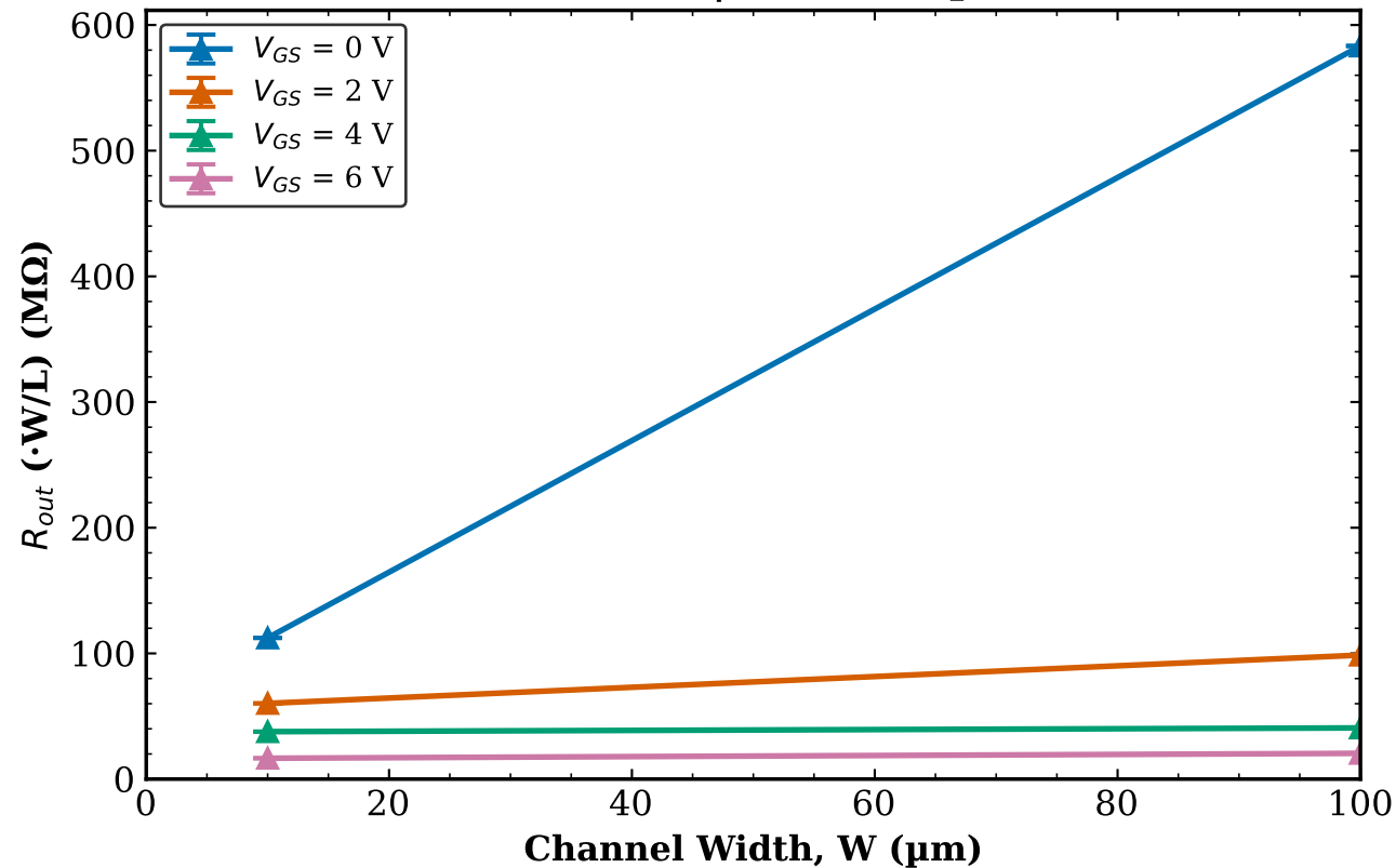
TFT1 Transistor 2 R_{out} vs W | L = 160\text{ }\mu\text{m}
